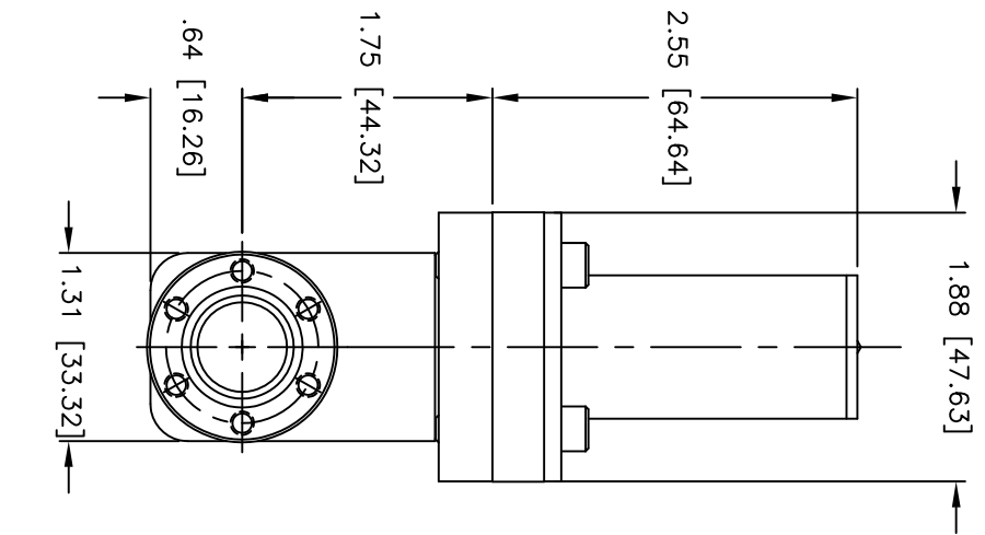
CARRIAGE SIDE
